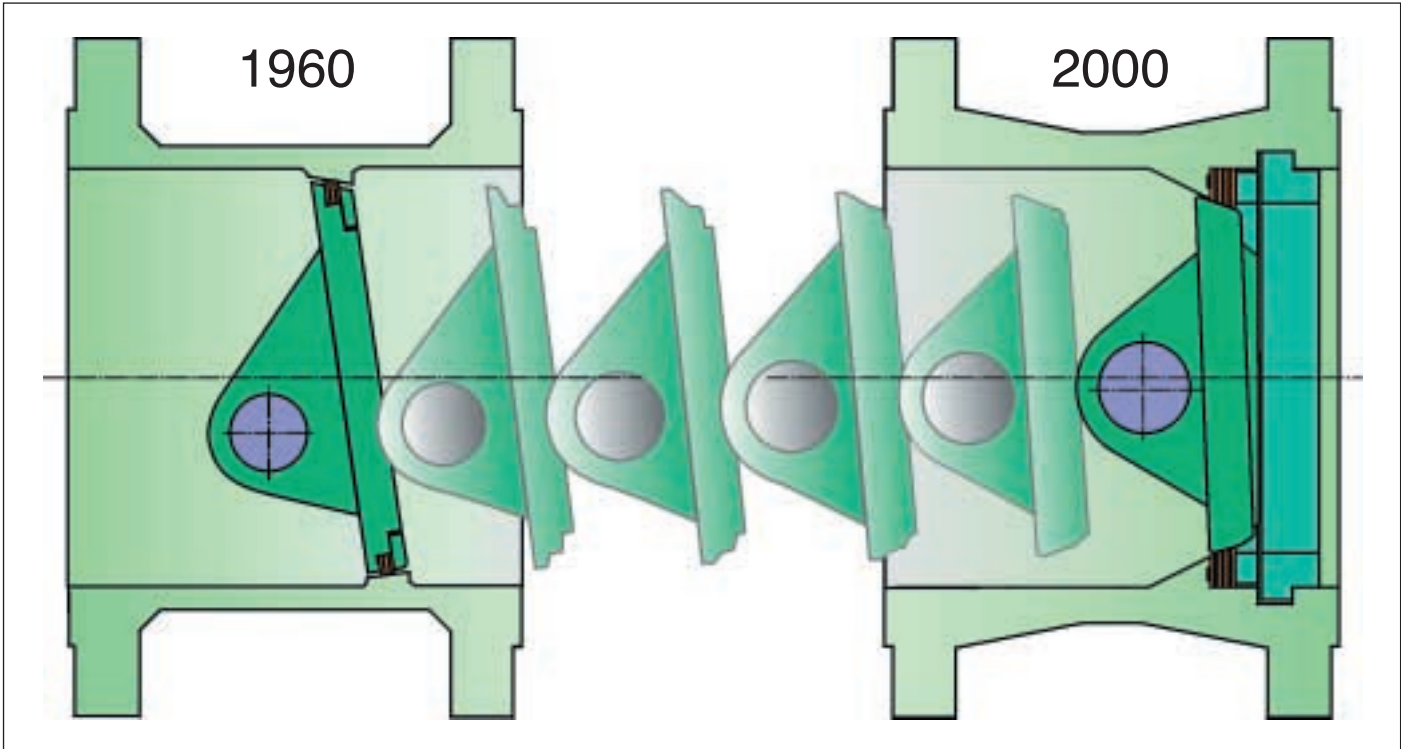
ADAMS created the Inclined Conical Sealing System and remains the leader in Rotary Tight Shut-Off Valve Technology
